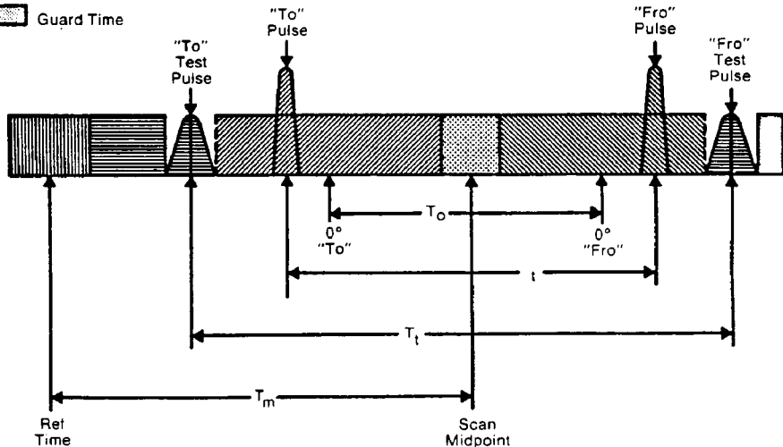
Figure 7. Azimuth Angle Scan Timing (Not to Scale)
