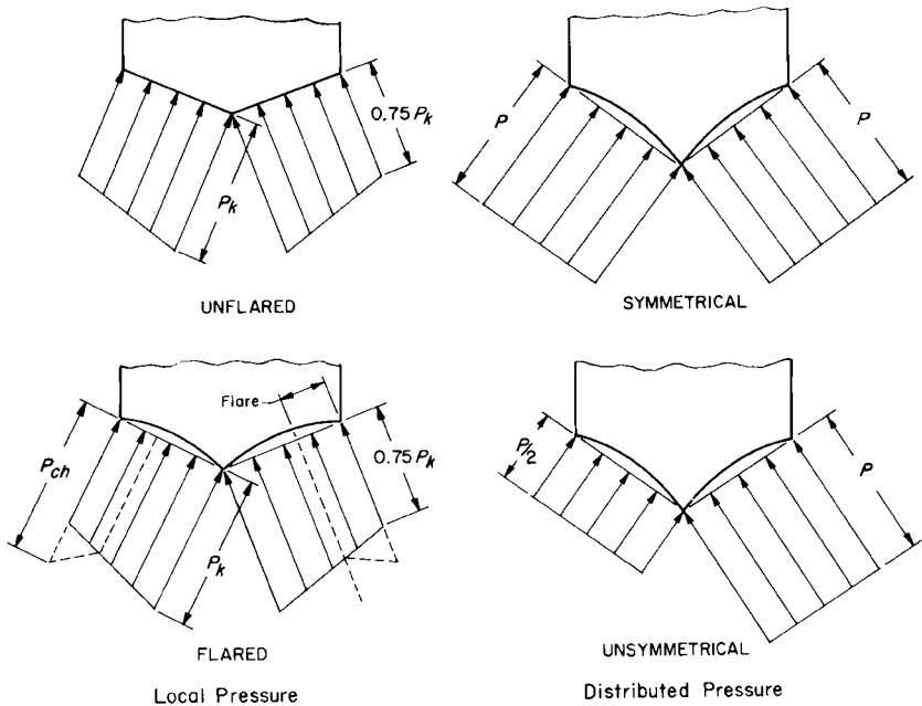
FIGURE 3. Transverse pressure distributions.
